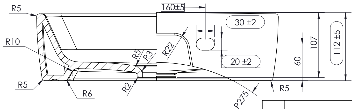
SECTION B-B
